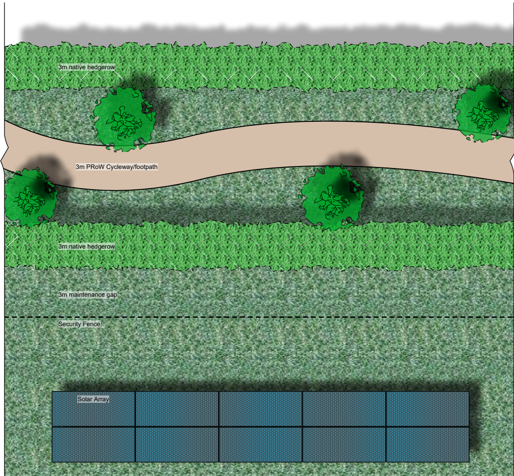
Plan View
